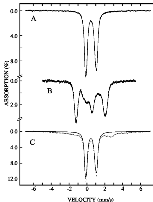
FIGURE 2: Mössbauer spectra of WT AI LS recorded at 4.2 K in an externally applied field (oriented parallel to the \gamma -beam) of (A) 40 mT and (B) 8 T. The solid line overlaid with the experimental data (hash marks) are simulations representing the contribution from the [4\text{Fe}-4\text{S}]^{2+} clusters using the parameters given in the text. The Mössbauer spectrum of WT RCN LS recorded at 4.2 K in an externally applied field (oriented parallel to the \gamma -beam) of 40 mT is shown in panel C. The simulation of the [4\text{Fe}-4\text{S}]^{2+} clusters, scaled to 70% of the total intensity of spectrum C is shown as a solid line.
